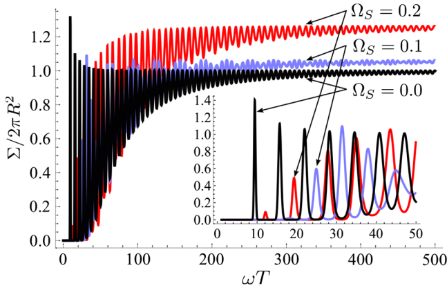
FIG. 2 (color online). Interferometer scale factor. Results for the two-dimensional case are shown with R = 10 and flat-top speed profile \Omega_p(\tau) = \pi/\omega T for 0 < \tau < \omega T . Plots for \Omega_S = 0, 0.1, 0.2 are shown in black, blue, and red. The inset shows the same data for 0 < \omega T < 50 .
