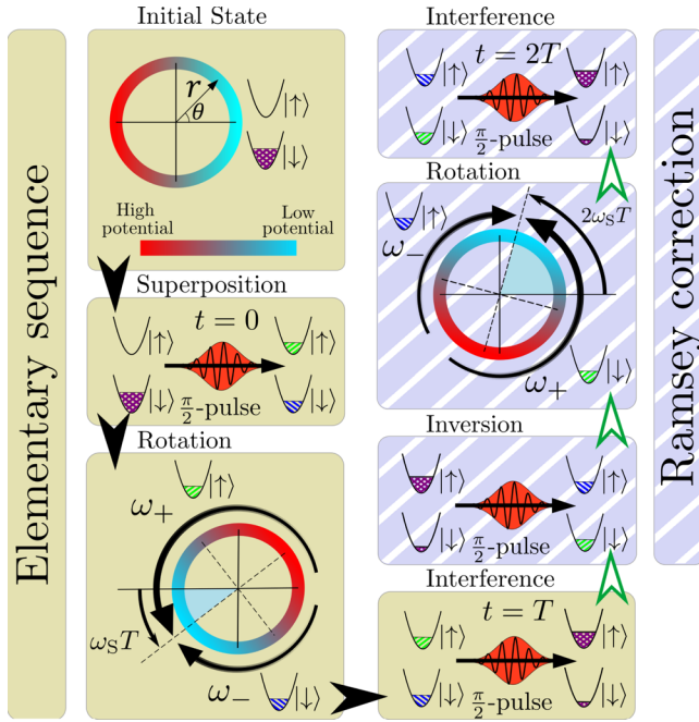
FIG. 1 (color online). Experimental sequence. The situation is depicted in an inertial frame. Starting with atoms prepared in |\downarrow\rangle located at \theta = 0 , a \pi/2 pulse generates a superposition of two nondegenerate internal states. Atoms in |\uparrow\rangle are then transported along a circular path in (anti-)clockwise direction. After a half revolution, a second pulse converts any phase shift into population difference, which is measured in the elementary sequence (black arrows). An extended Ramsey sequence (green arrows) can be used to achieve full common path operation. Here, the \pi/2 pulse at time T is extended to a \pi pulse, fully inverting the atomic states. Transport is continued such that all atoms complete a full revolution before converting and measuring the phase difference at time 2T .
